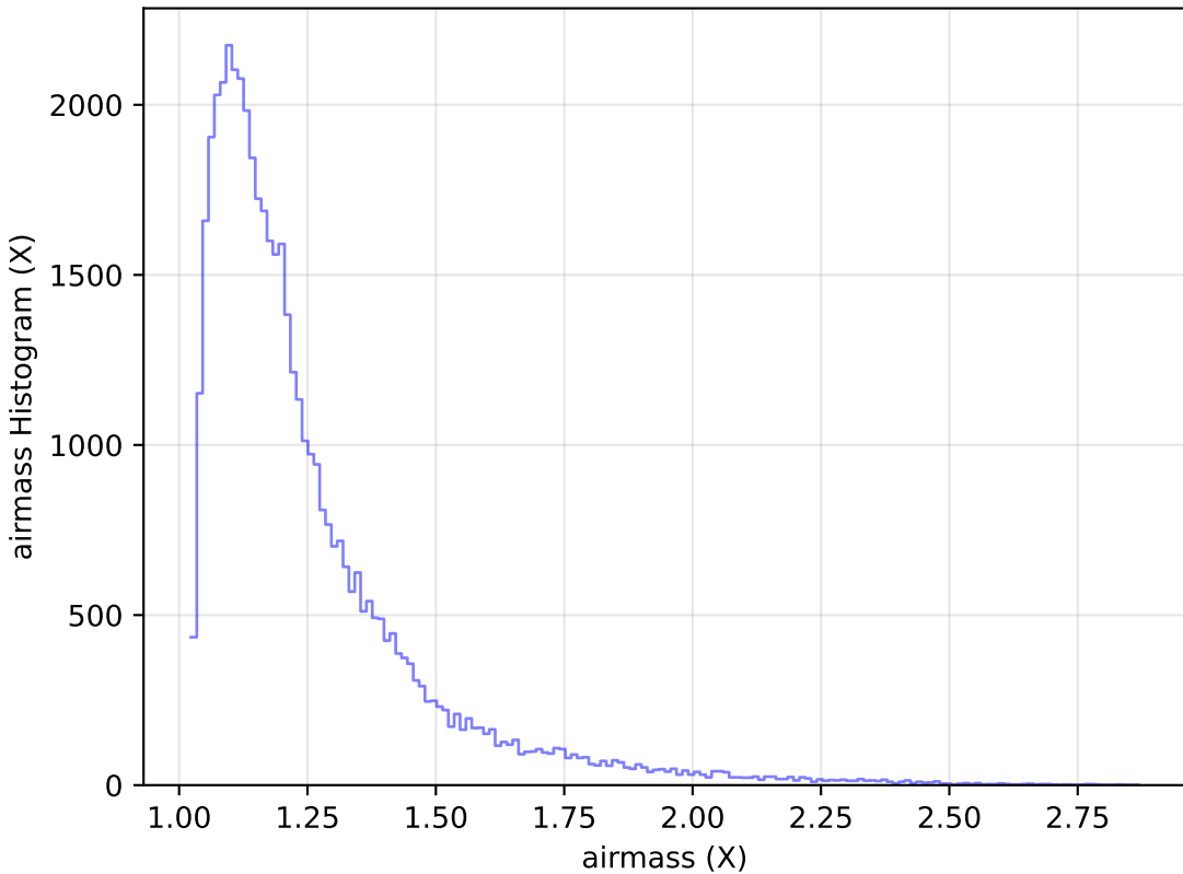
too_10_4v3.4_10yrs Yr 1 y band: airmass Histogram
