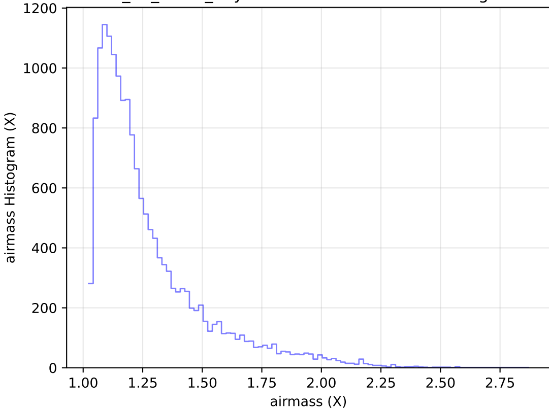
too_10_4v3.4_10yrs Yr 1 u band: airmass Histogram
