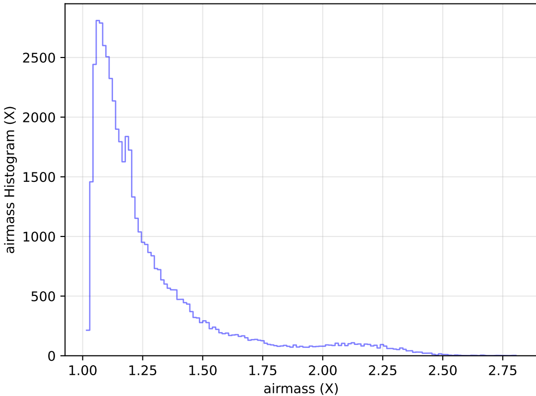
too_10_4v3.4_10yrs Yr 1 r band: airmass Histogram
