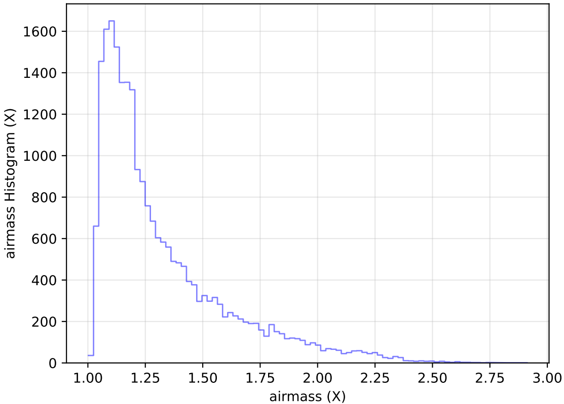
too_10_4v3.4_10yrs Yr 1 g band: airmass Histogram
