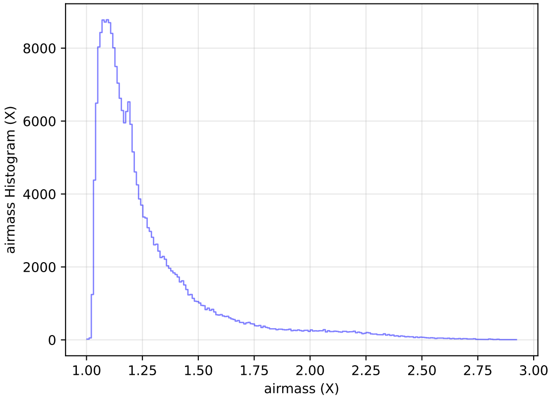
too_10_4v3.4_10yrs Yr 1 all bands: airmass Histogram
