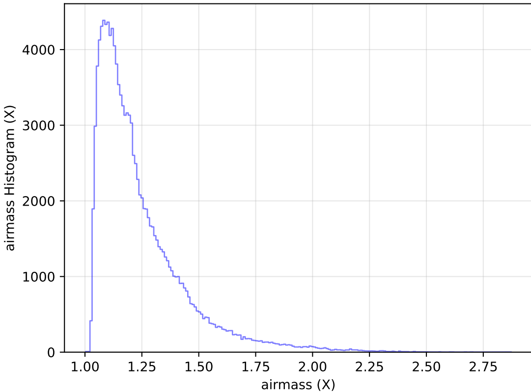
too_10_4v3.4_10yrs WFD u band: airmass Histogram
