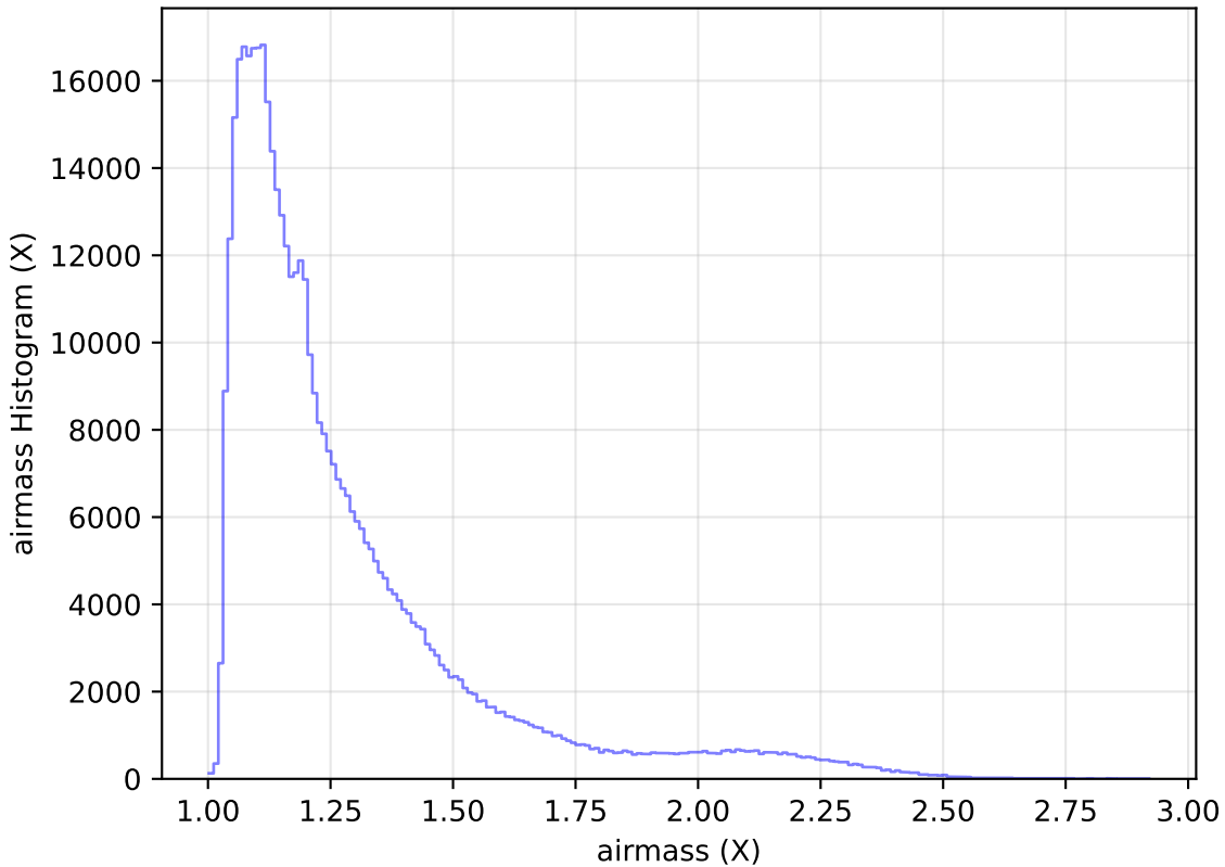
too_10_4v3.4_10yrs WFD r band: airmass Histogram
