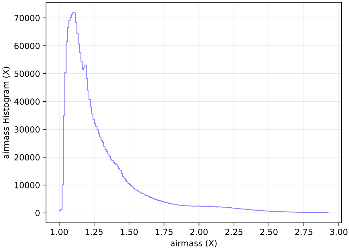
too_10_4v3.4_10yrs WFD all bands: airmass Histogram
