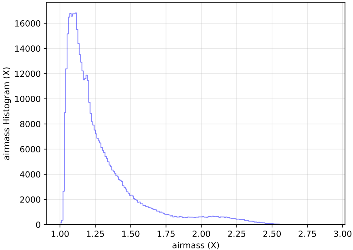
too_10_4v3.4_10yrs All sky r band: airmass Histogram
