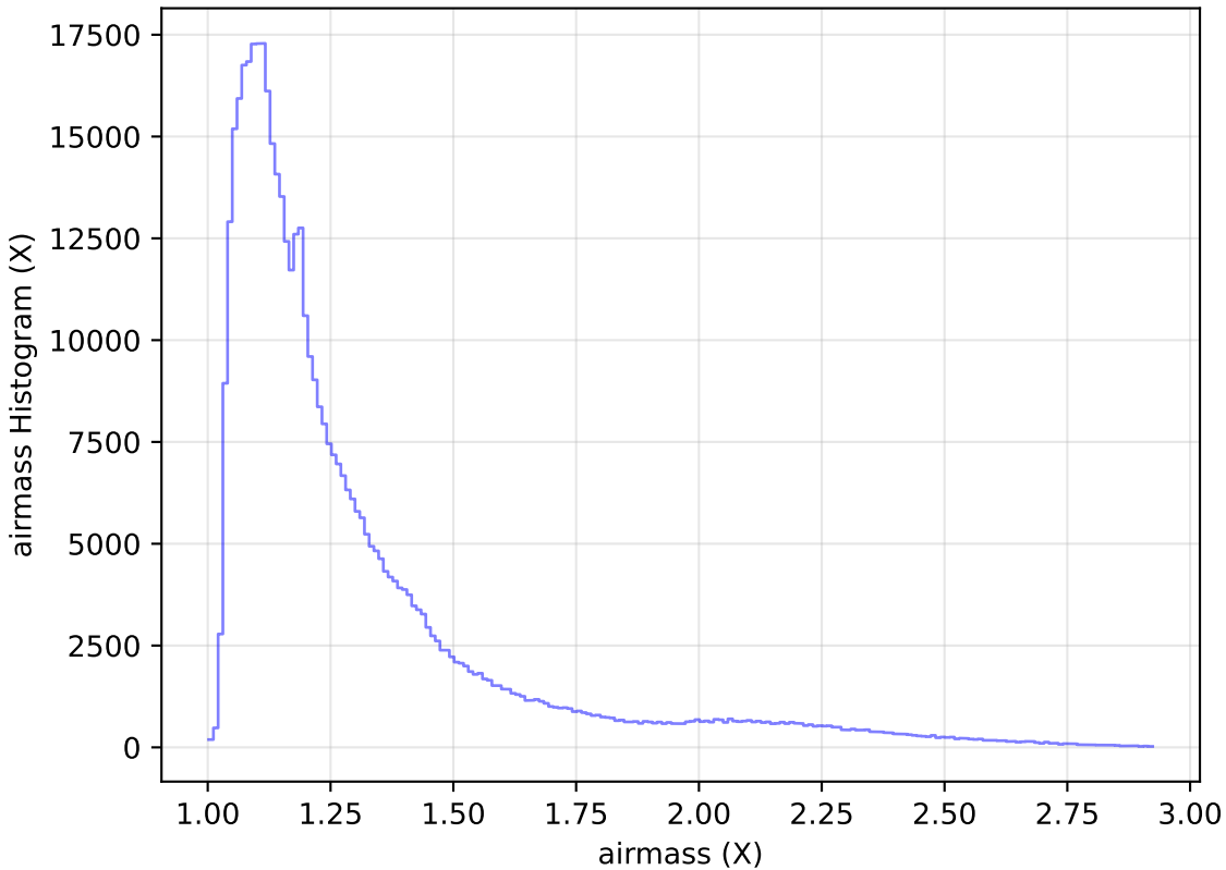
too_10_4v3.4_10yrs All sky i band: airmass Histogram
