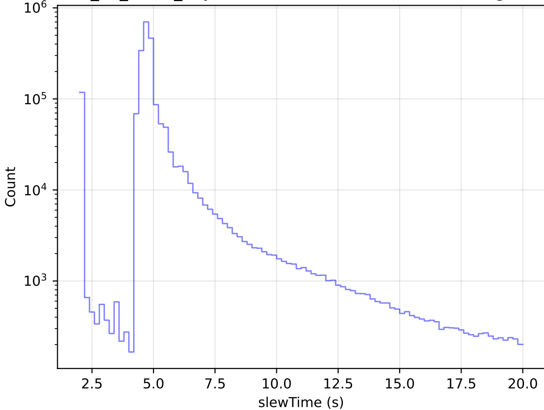
too_10_4v3.4_10yrs All visits: Zoom Slew Time Histogram
