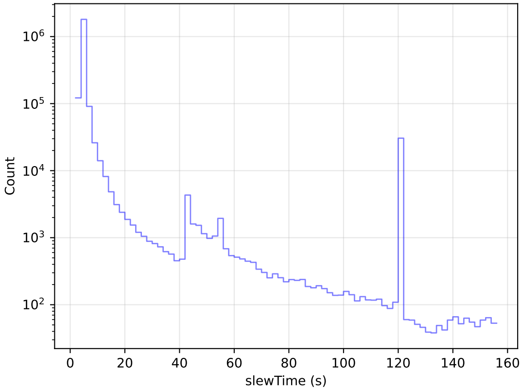
too_10_4v3.4_10yrs All visits: Slew Time Histogram
