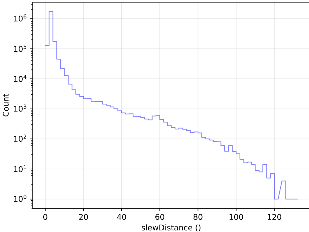
too_10_4v3.4_10yrs All visits: Slew Distance Histogram
