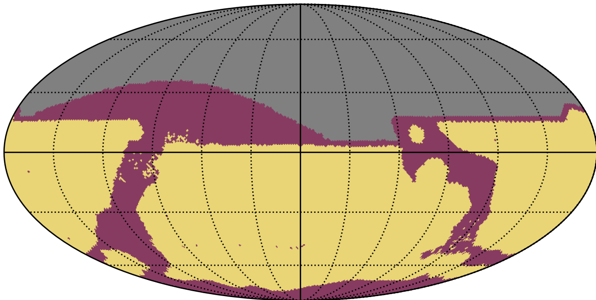
too_10_4v3.4_10yrs All sky: RapidRevisits
