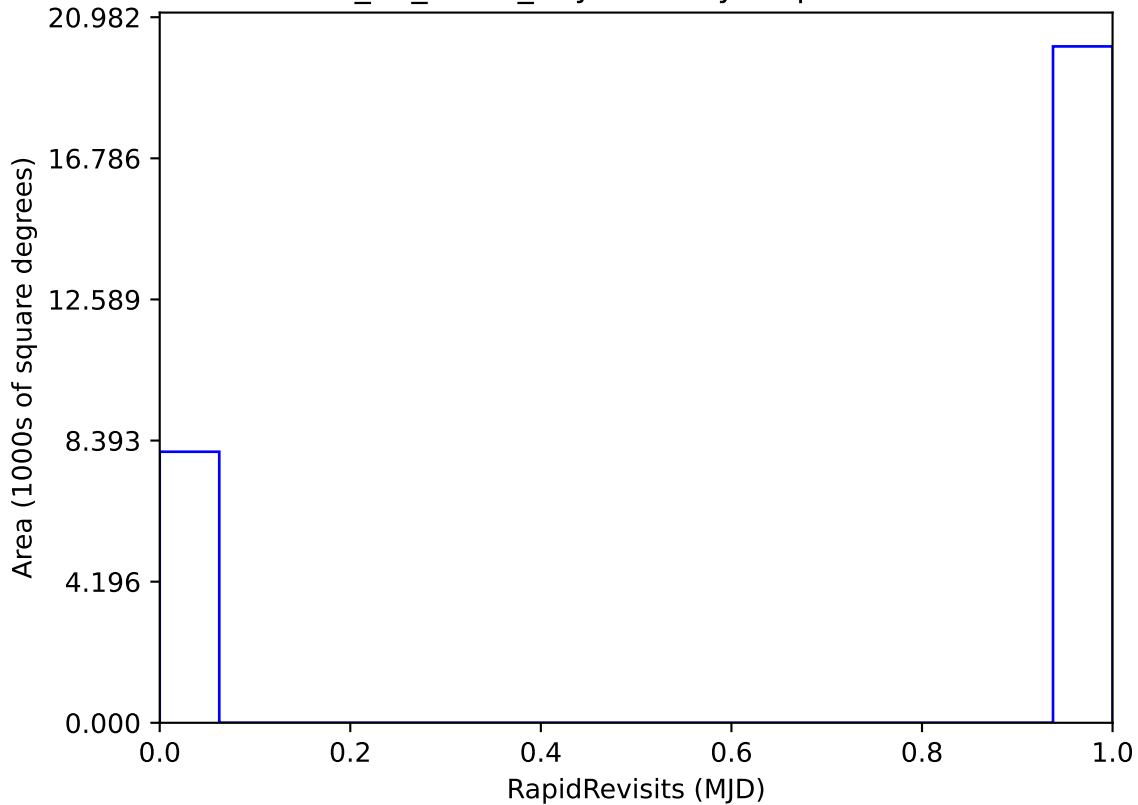
too_10_4v3.4_10yrs All sky: RapidRevisits
