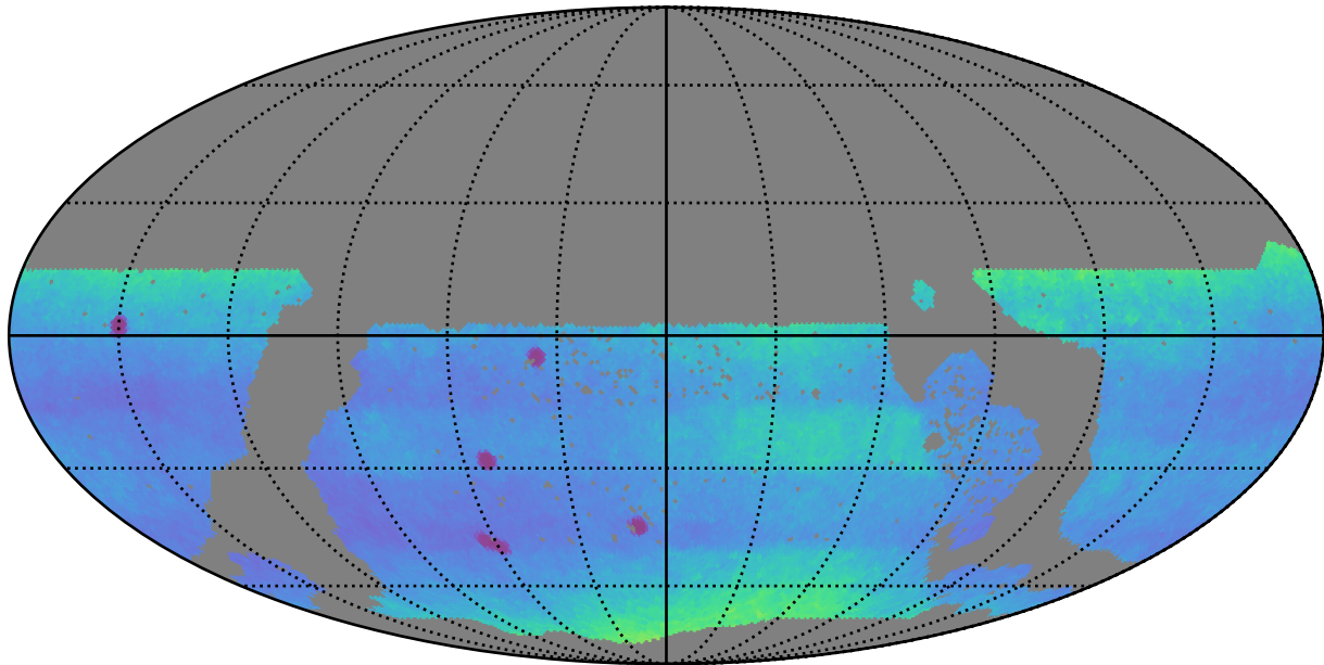
too_10_4v3.4_10yrs WFD: Proper Motion Uncert @ 24.0
