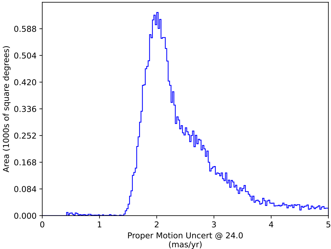
too_10_4v3.4_10yrs All sky: Proper Motion Uncert @ 24.0
