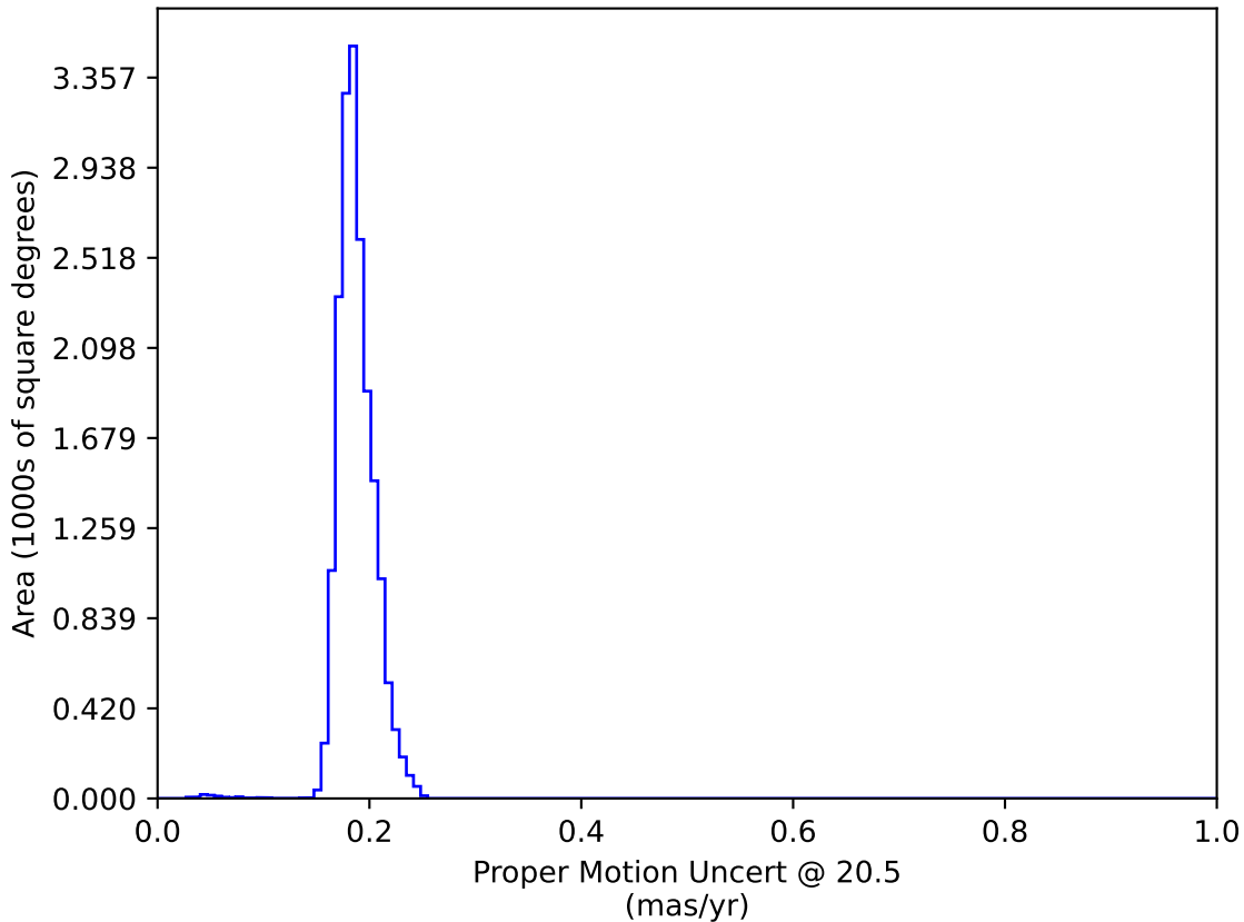
too_10_4v3.4_10yrs WFD: Proper Motion Uncert @ 20.5
