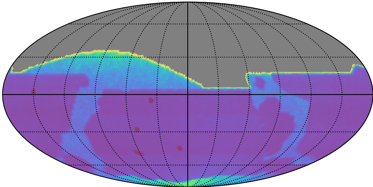
too_10_4v3.4_10yrs All sky: Proper Motion Uncert @ 20.5
