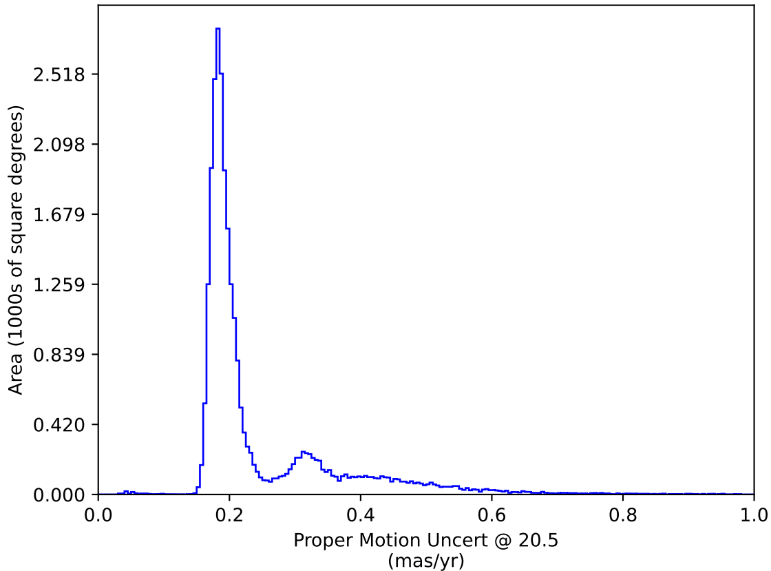
too_10_4v3.4_10yrs All sky: Proper Motion Uncert @ 20.5
