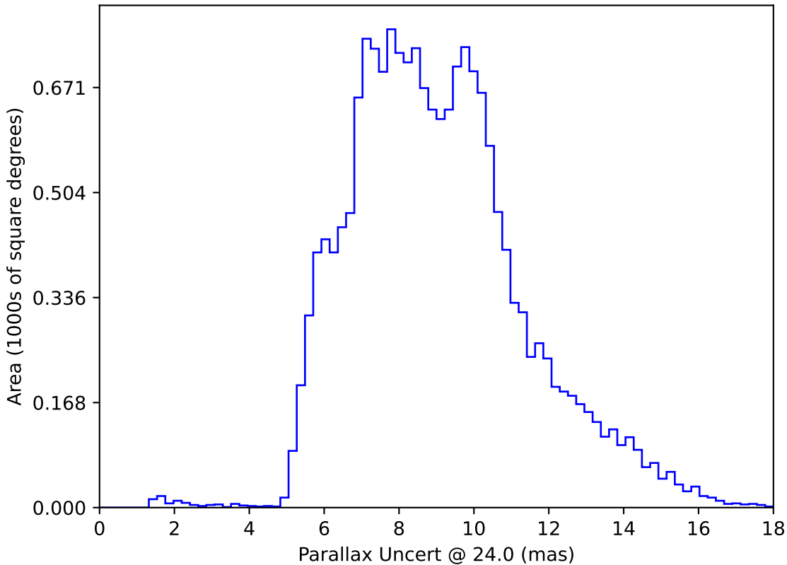
too_10_4v3.4_10yrs WFD: Parallax Uncert @ 24.0
