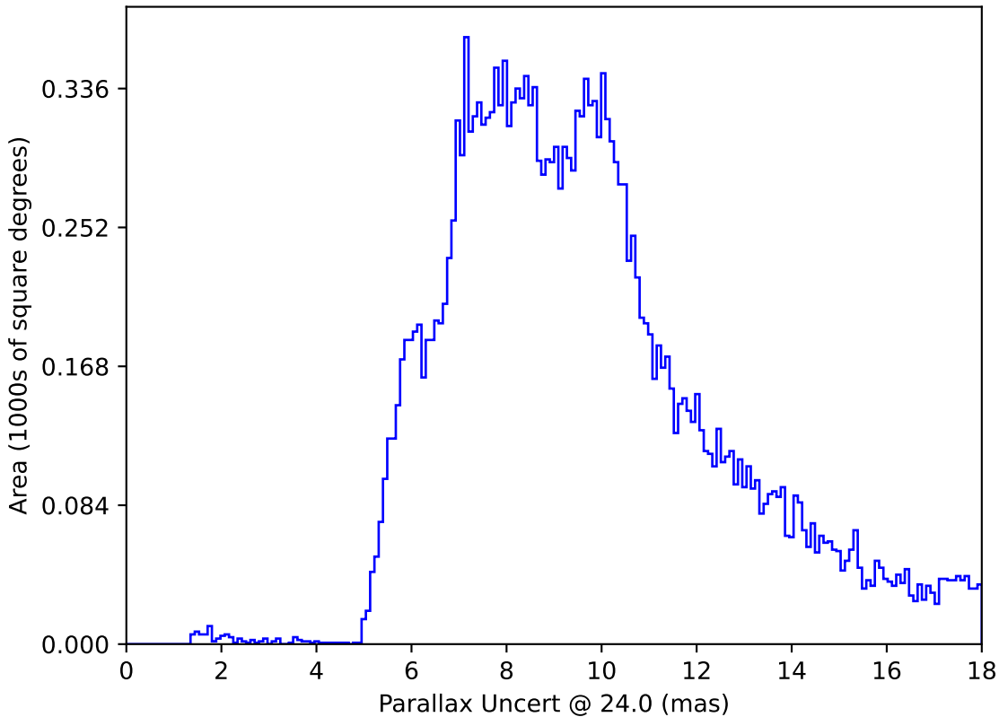
too_10_4v3.4_10yrs All sky: Parallax Uncert @ 24.0
