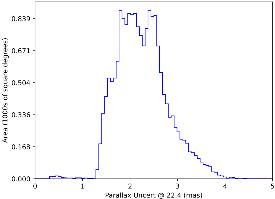
too_10_4v3.4_10yrs WFD: Parallax Uncert @ 22.4
