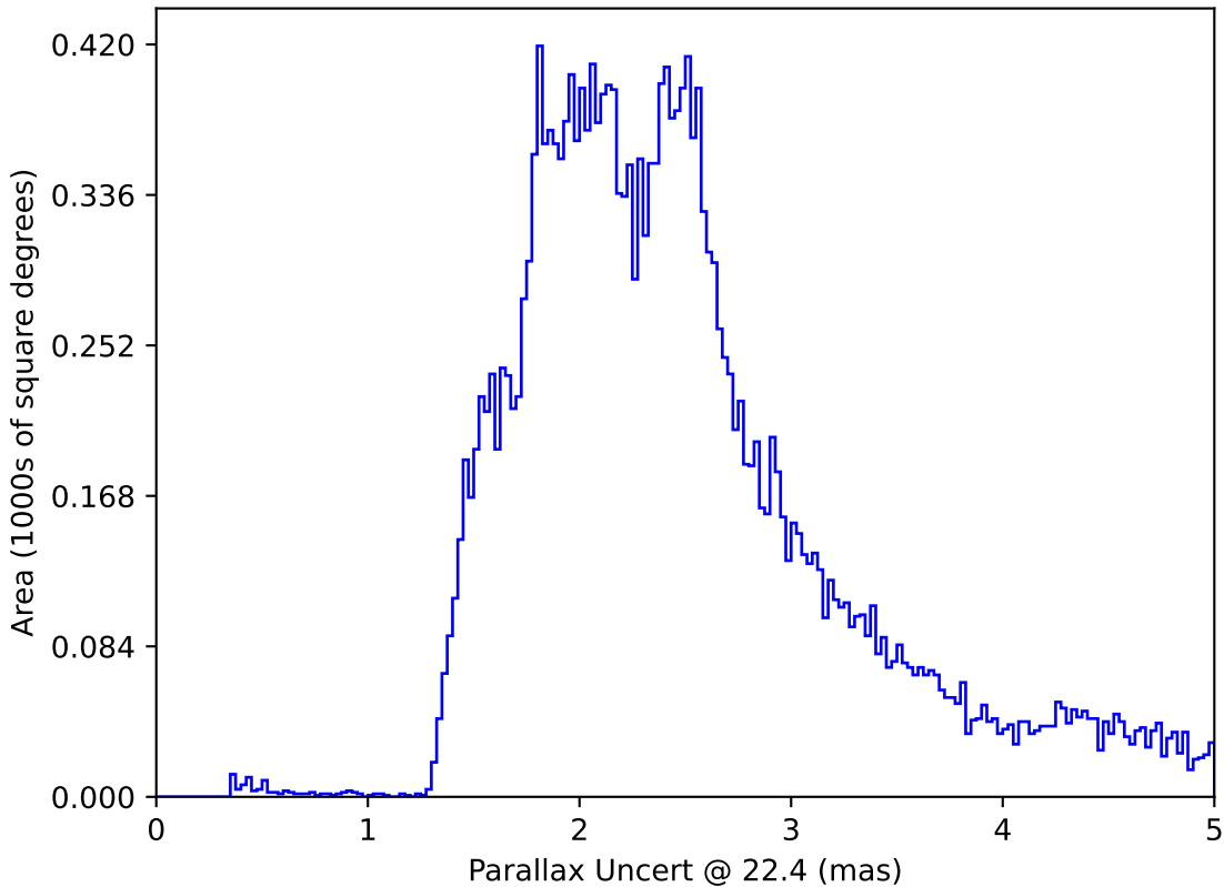
too_10_4v3.4_10yrs All sky: Parallax Uncert @ 22.4
