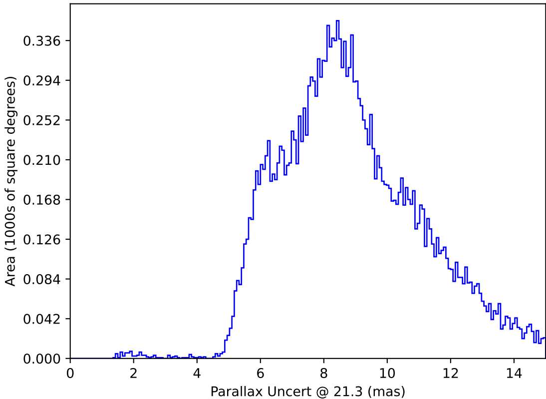
too_10_4v3.4_10yrs All sky y band only: Parallax Uncert @ 21.3
