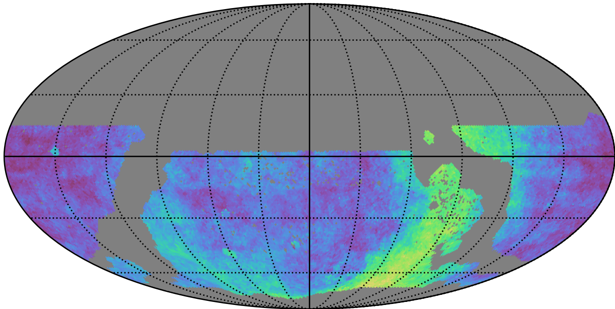
too_10_4v3.4_10yrs WFD: Parallax Coverage @ 24.0
