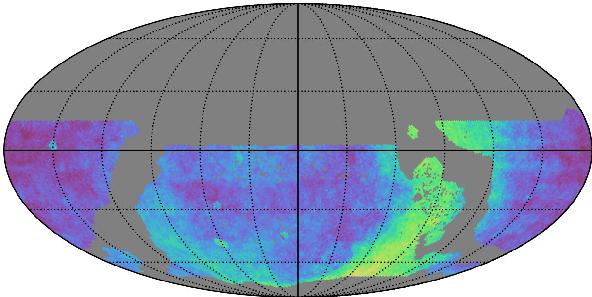
too_10_4v3.4_10yrs WFD: Parallax Coverage @ 22.4
