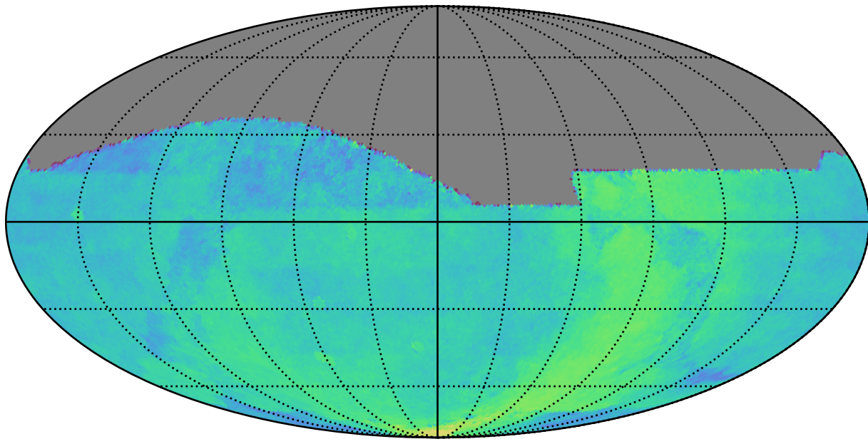
too_10_4v3.4_10yrs All sky: Parallax Coverage @ 22.4
