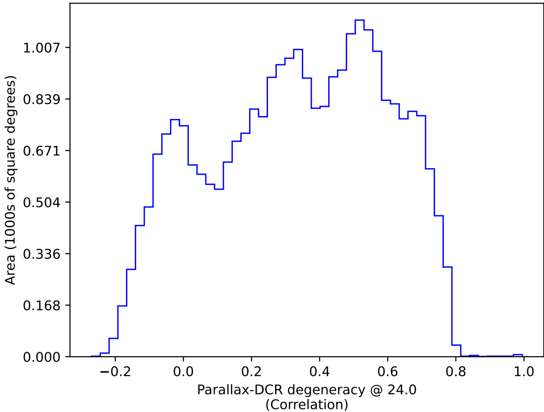
too_10_4v3.4_10yrs All sky: Parallax-DCR degeneracy @ 24.0
