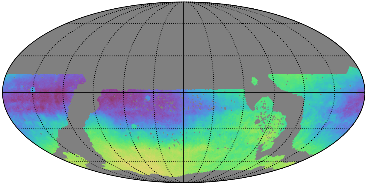
too_10_4v3.4_10yrs WFD: Parallax-DCR degeneracy @ 22.4
