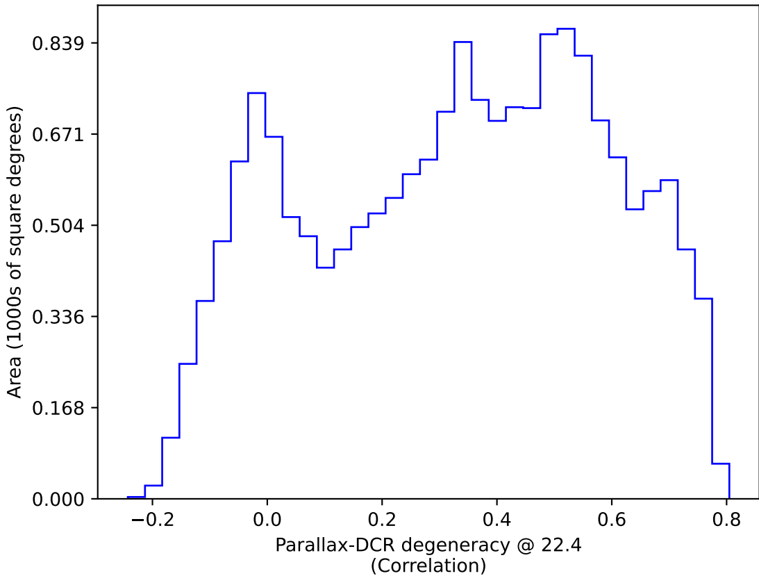
too_10_4v3.4_10yrs WFD: Parallax-DCR degeneracy @ 22.4
