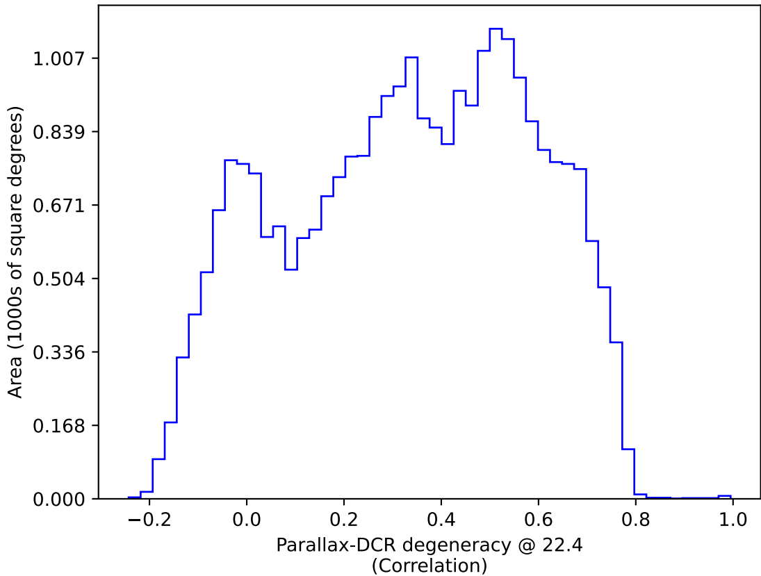
too_10_4v3.4_10yrs All sky: Parallax-DCR degeneracy @ 22.4
