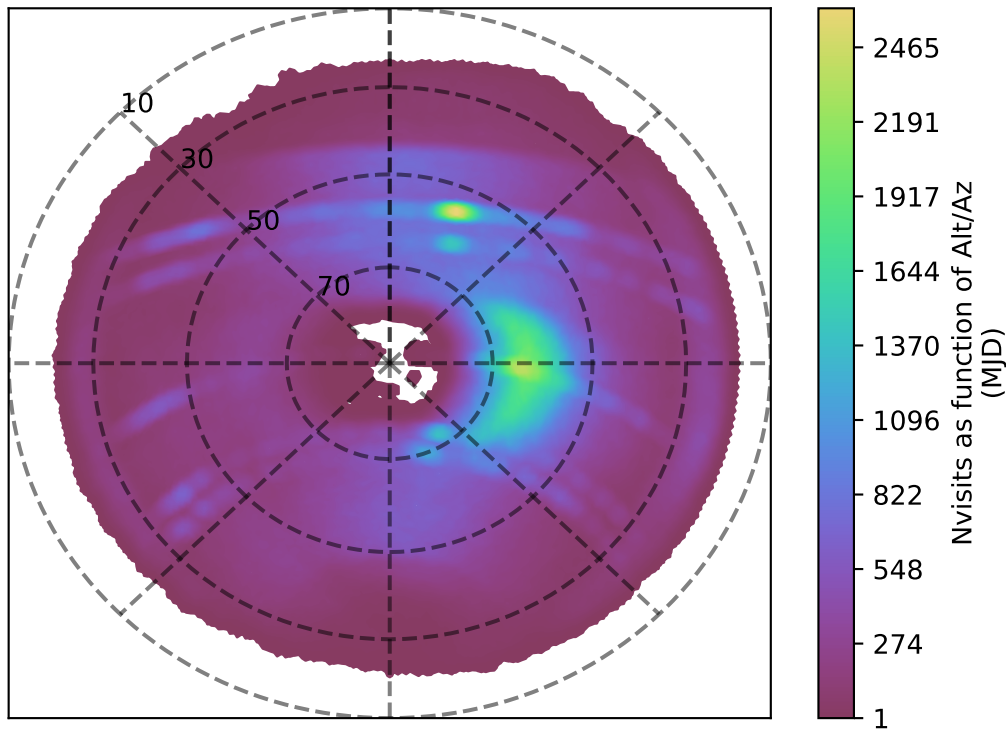
too_10_4v3.4_10yrs z band: Nvisits as function of Alt/Az
