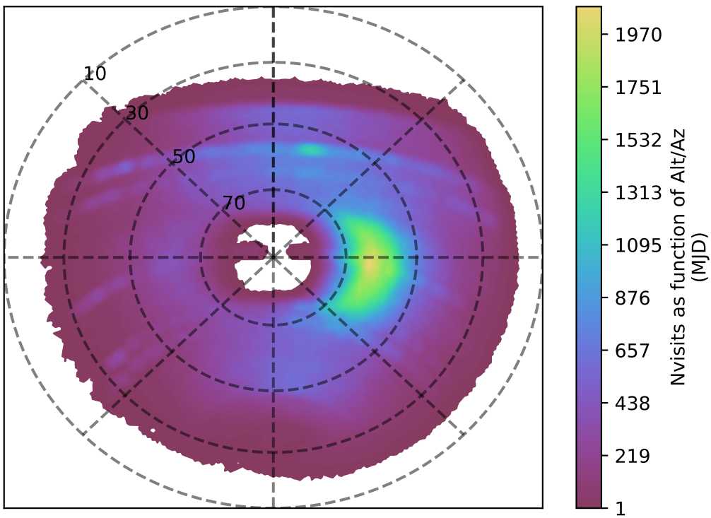
too_10_4v3.4_10yrs y band: Nvisits as function of Alt/Az
