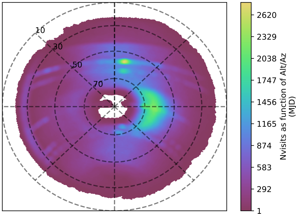
too_10_4v3.4_10yrs r band: Nvisits as function of Alt/Az
