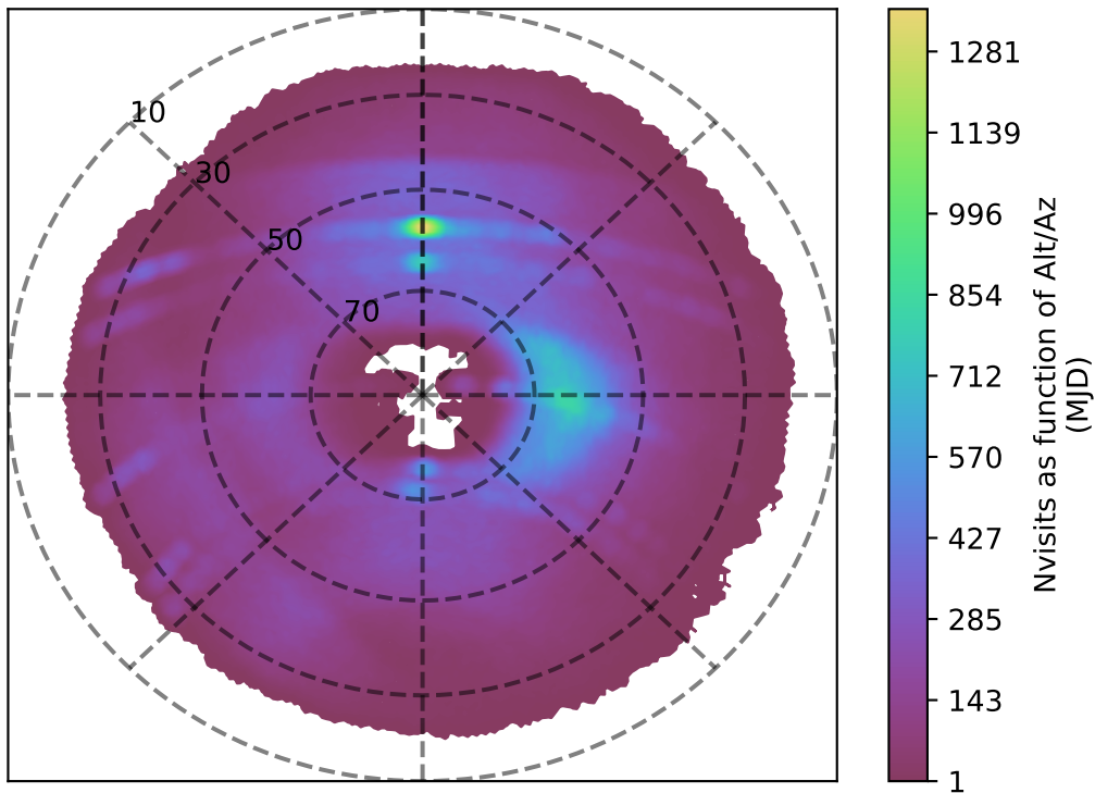
too_10_4v3.4_10yrs g band: Nvisits as function of Alt/Az
