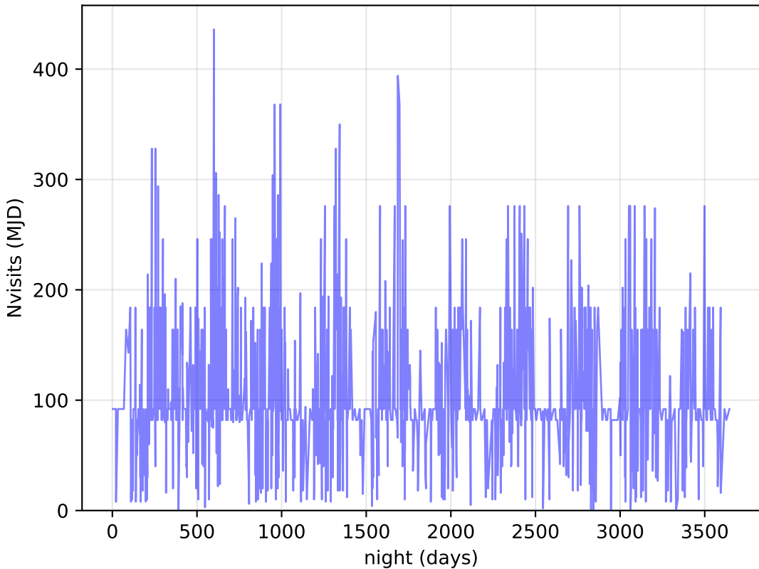
too_10_4v3.4_10yrs DDF: Nvisits
