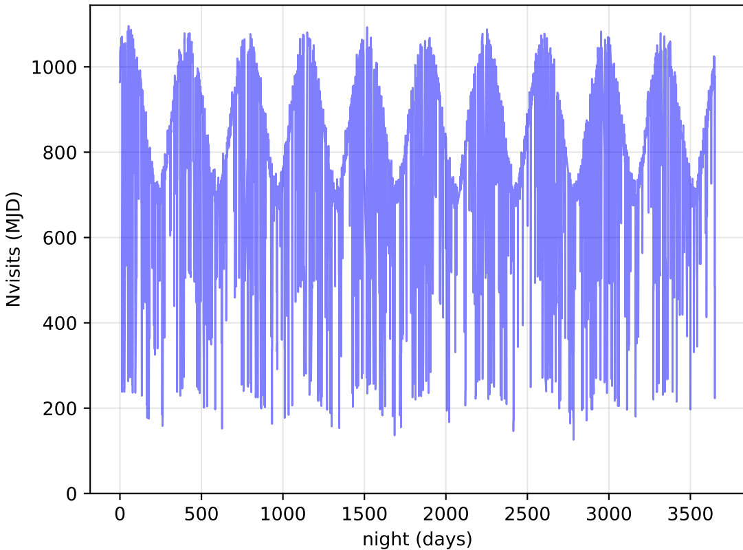
too_10_4v3.4_10yrs All visits: Nvisits
