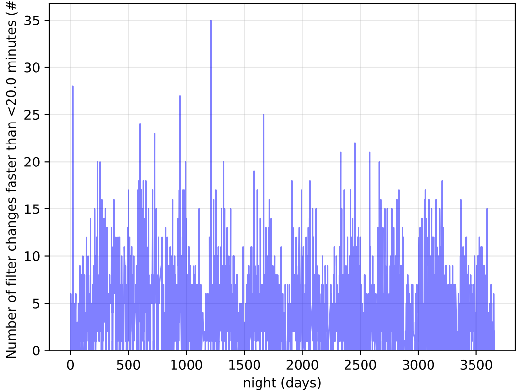
too_10_4v3.4_10yrs Per Night: Number of filter changes faster than <20.0 minutes
