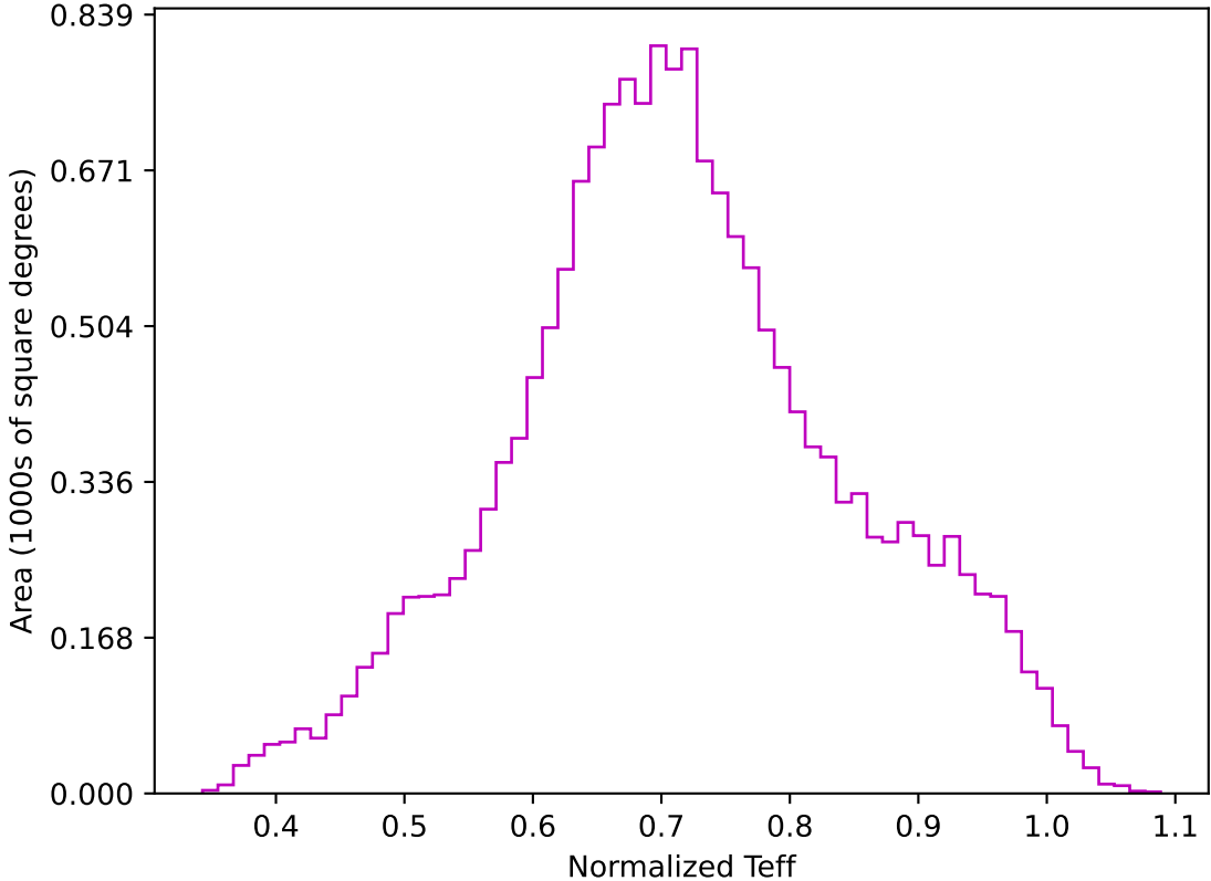
too_10_4v3.4_10yrs WFD z band: Normalized Teff
