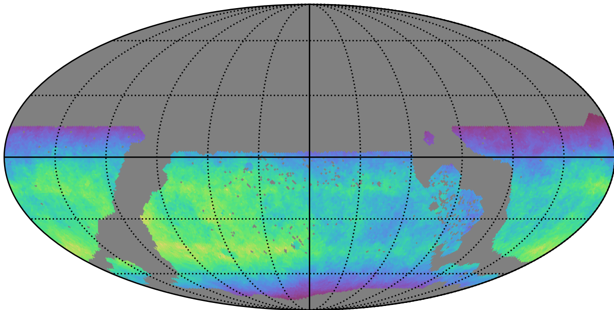
too_10_4v3.4_10yrs WFD y band: Normalized Teff
