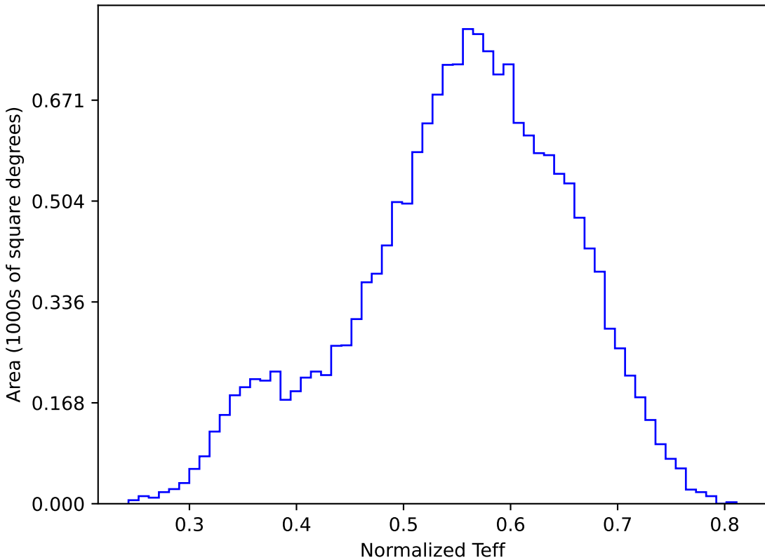
too_10_4v3.4_10yrs WFD y band: Normalized Teff
