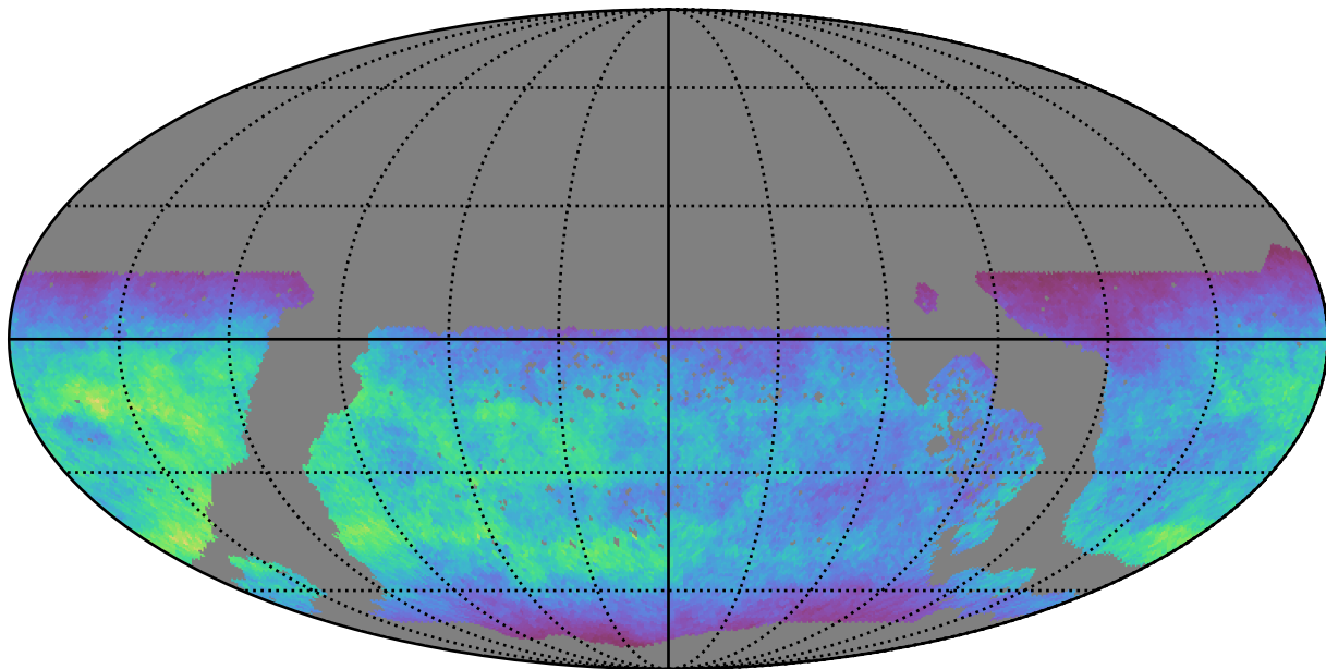
too_10_4v3.4_10yrs WFD u band: Normalized Teff
