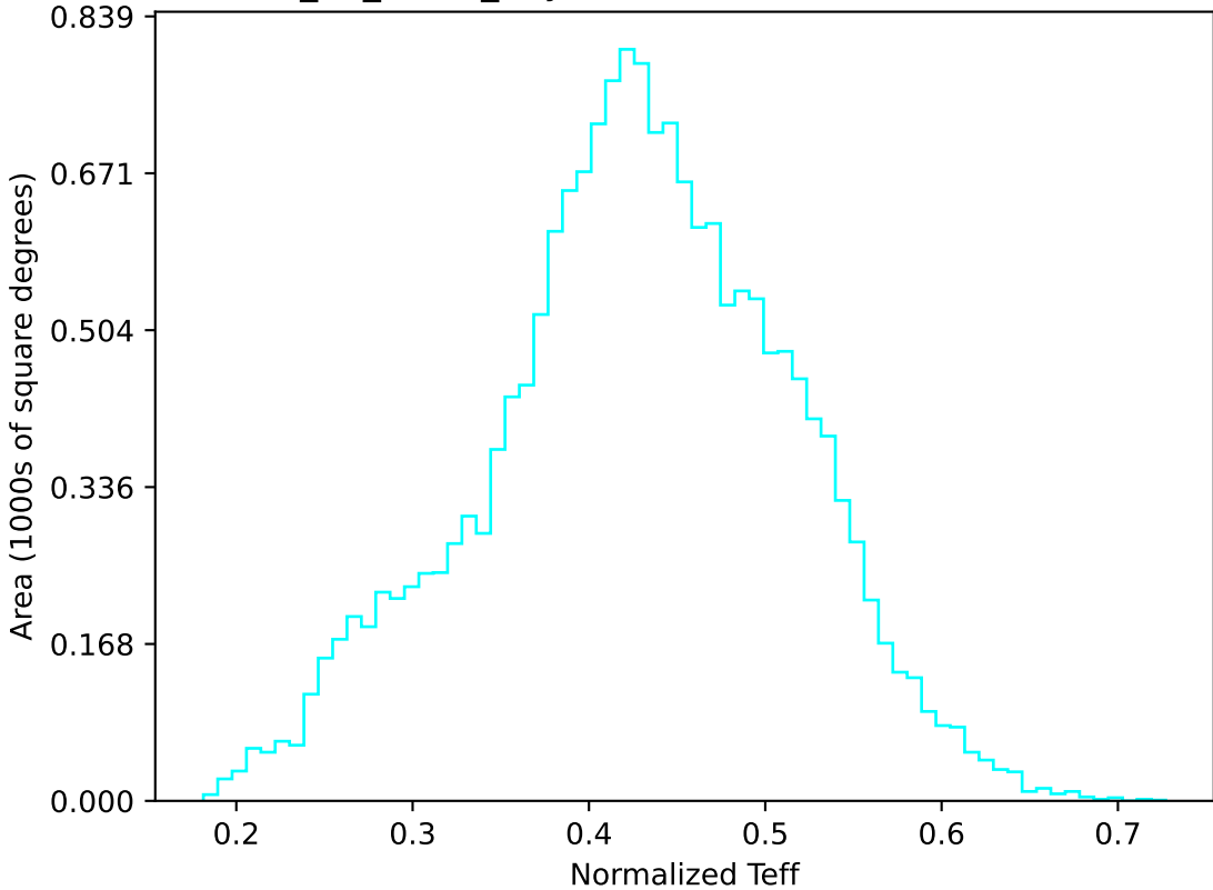
too_10_4v3.4_10yrs WFD u band: Normalized Teff
