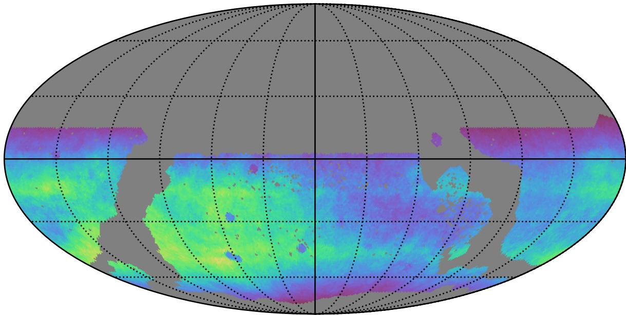
too_10_4v3.4_10yrs WFD r band: Normalized Teff
