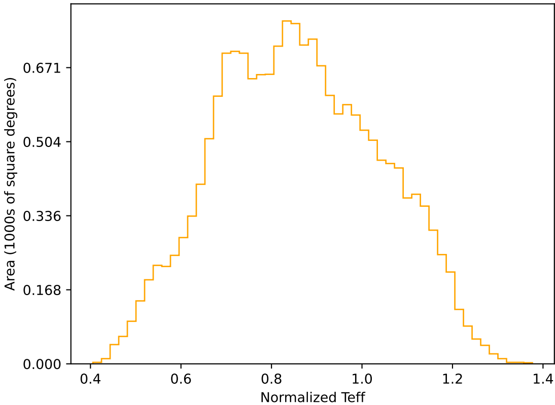
too_10_4v3.4_10yrs WFD r band: Normalized Teff
