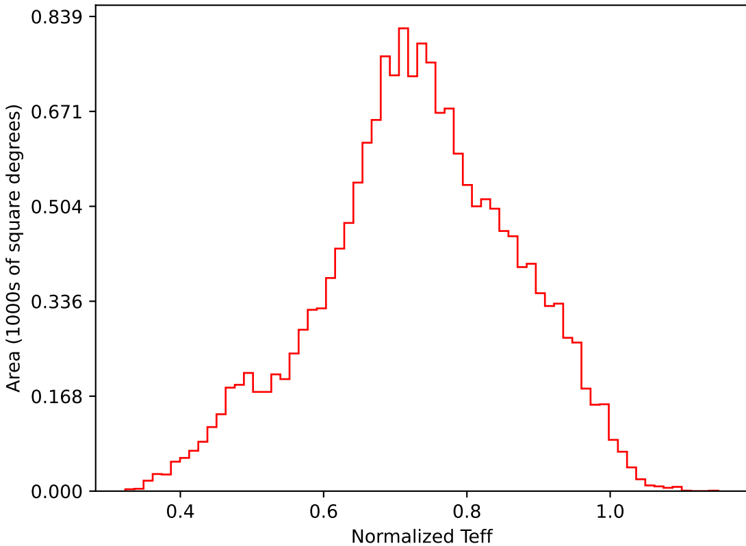
too_10_4v3.4_10yrs WFD i band: Normalized Teff
