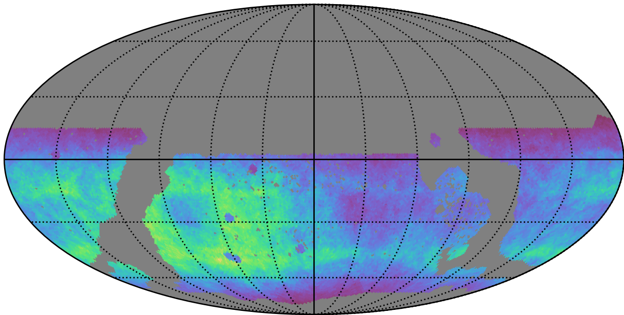
too_10_4v3.4_10yrs WFD g band: Normalized Teff
