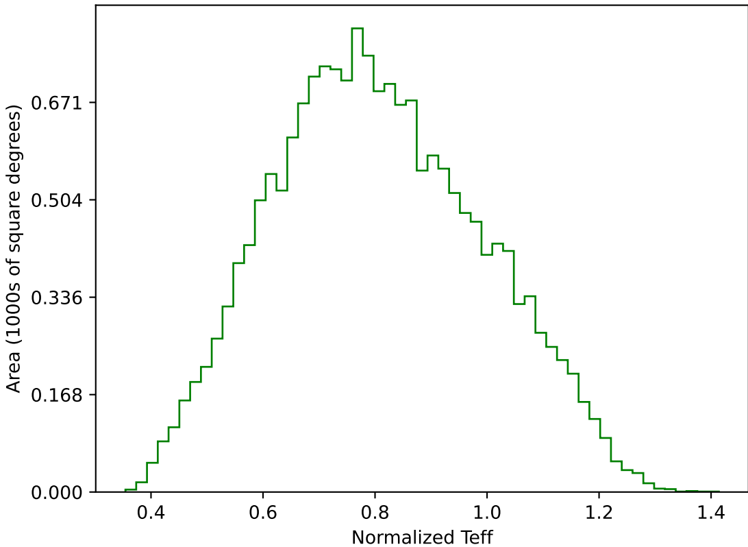
too_10_4v3.4_10yrs WFD g band: Normalized Teff
