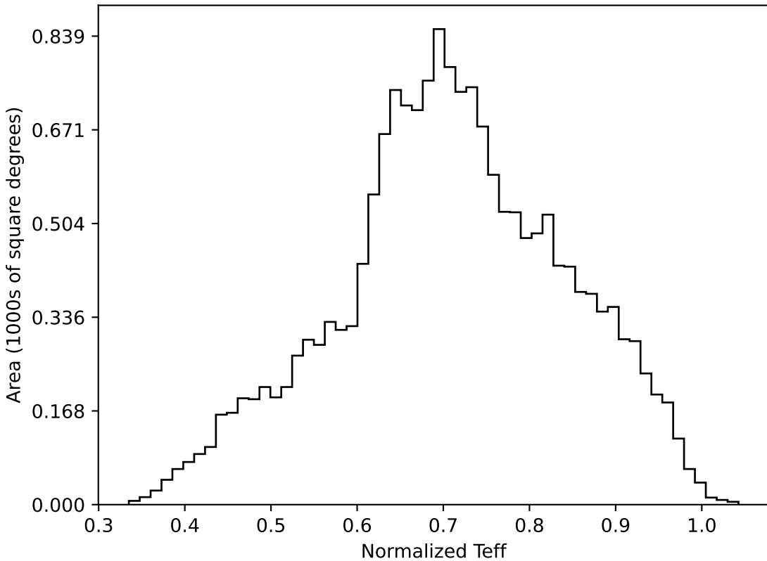
too_10_4v3.4_10yrs WFD all bands: Normalized Teff
